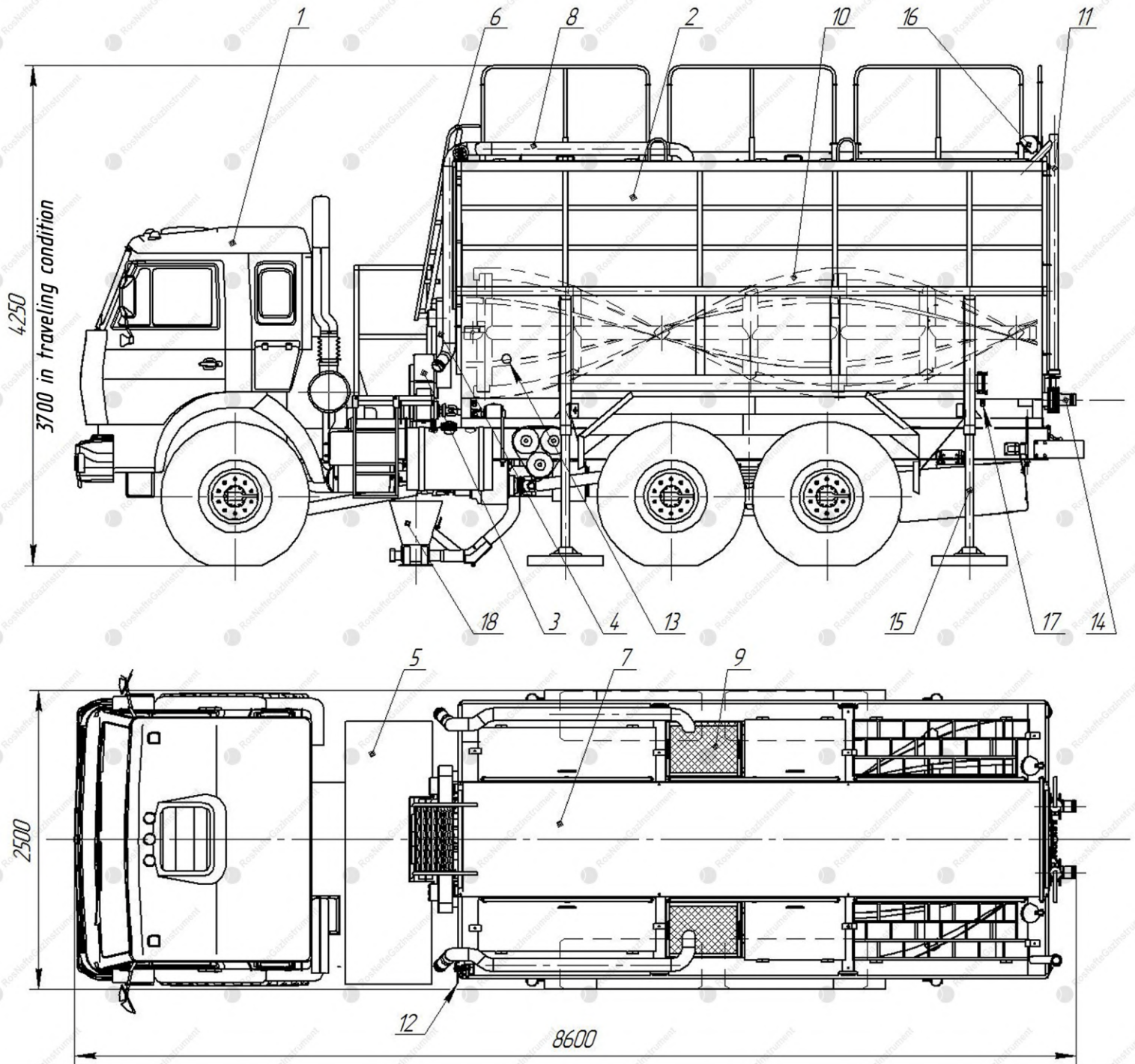
Pic. 1 USO-20R1-02 The mixing-averaging unit.
